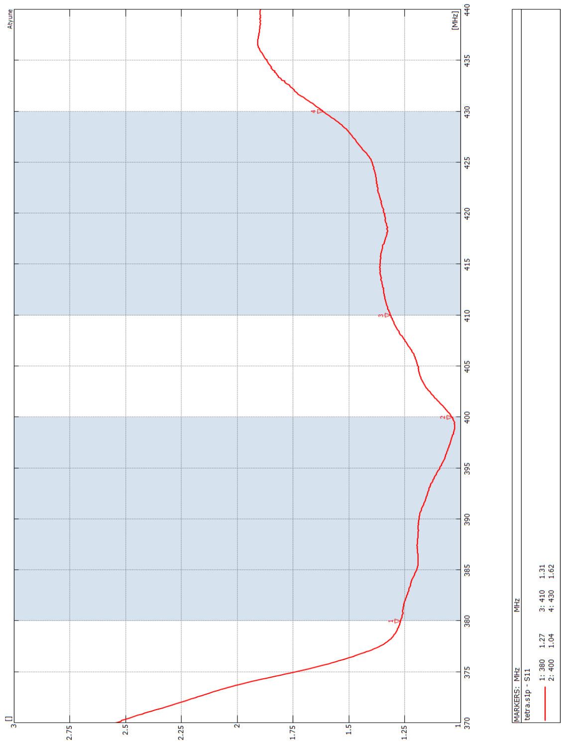
TETRA VSWR Plot
