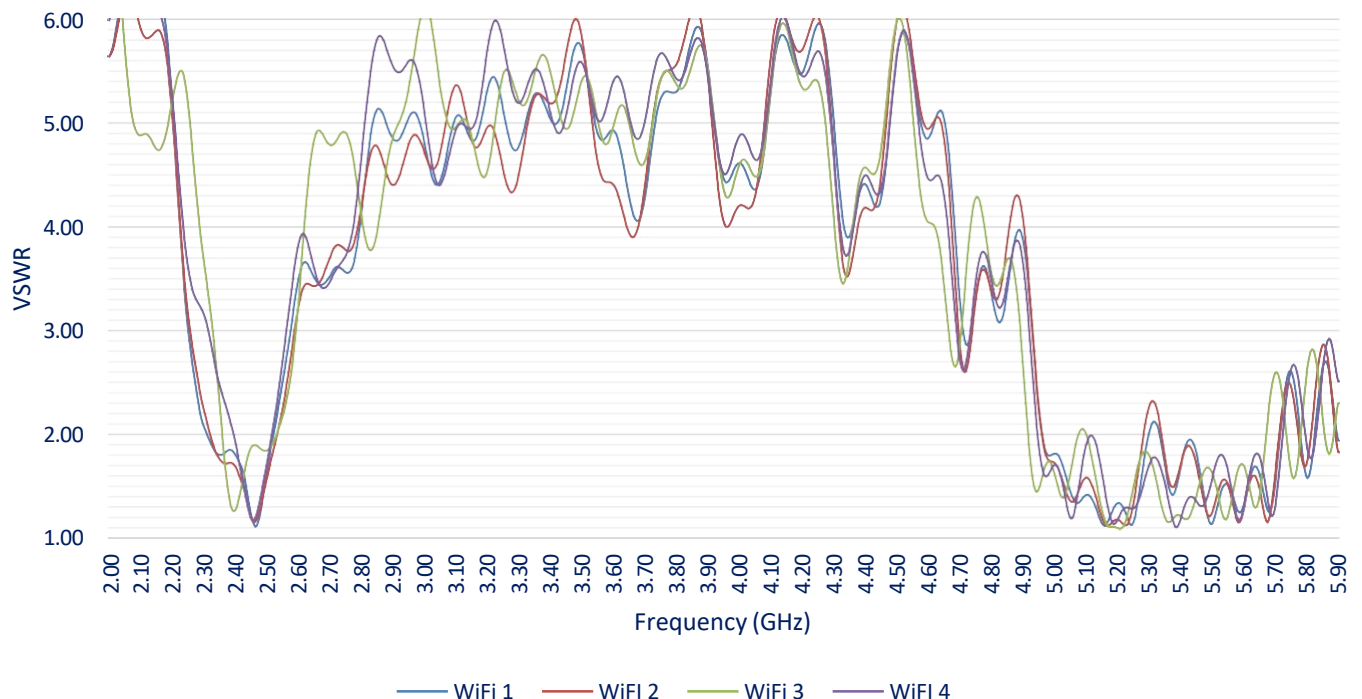
WiFi VSWR
