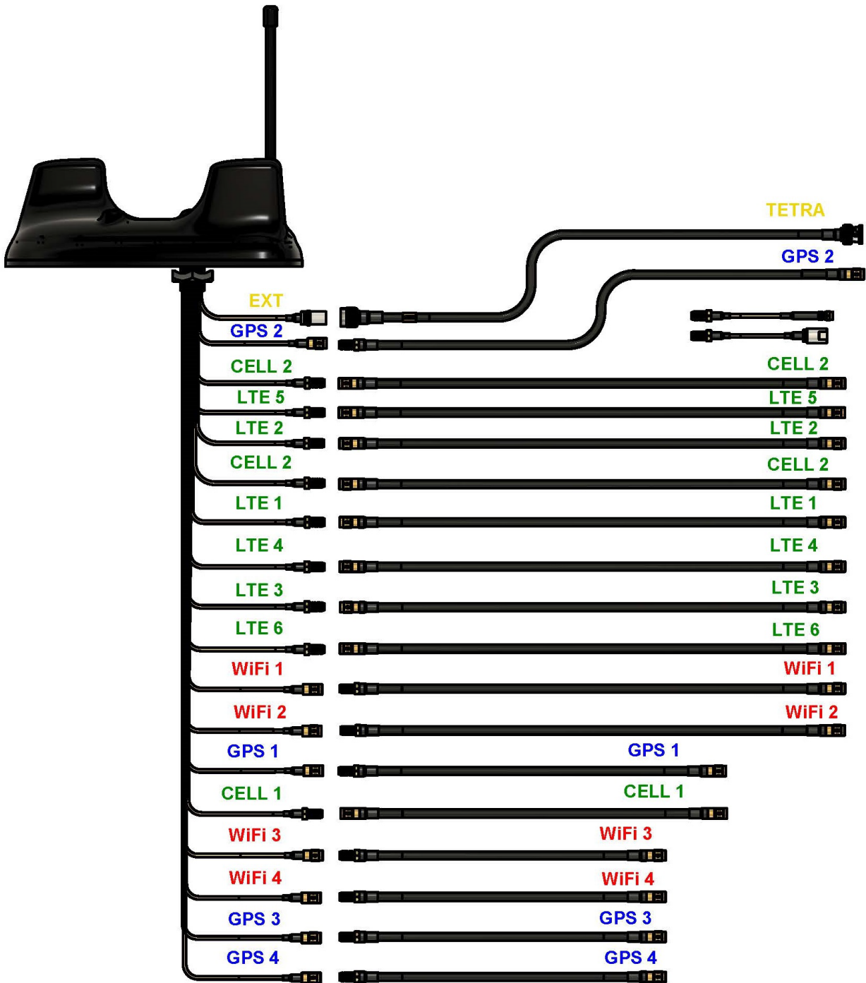
Cable Diagram
