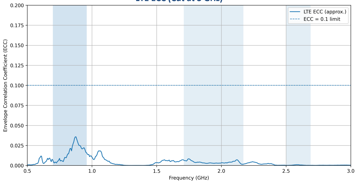
LTE ECC (Cut at 3 GHz)
