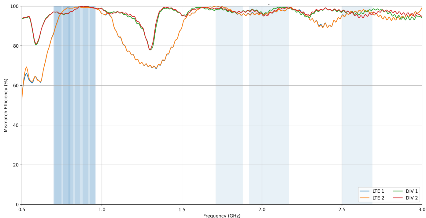
LTE / DIV Ports – Mismatch Efficiency
