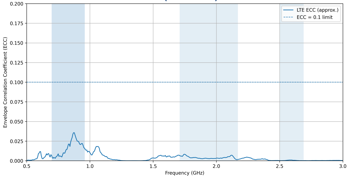
LTE ECC (Cut at 3 GHz)
